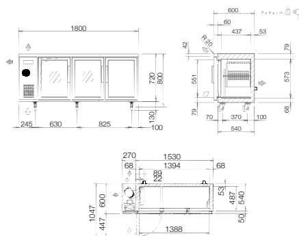
BR-1861HP(AUH) [SLIMLINE TYPE]
