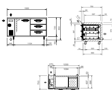
SUR-1571HP(AUH)-DW [DRAWER TYPE]
