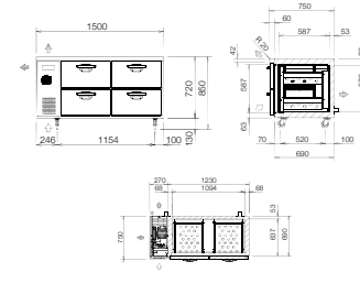
SUR-1571HP(AUH)-NN [DRAWER TYPE]
