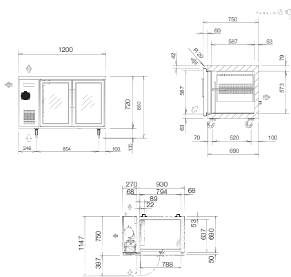
BR-1271HP(AUH) [LARGE CAPACITY TYPE]
