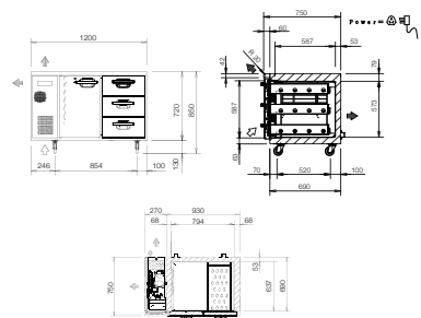
SUR-1271HP(AUH)-DW [DRAWER TYPE]
