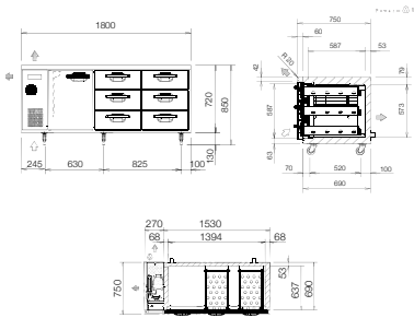
SUR-1871HP(AUH)-DWW [DRAWER TYPE]
