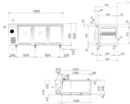
BR-1871HP(AUH) [LARGE CAPACITY TYPE]
