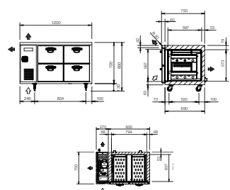
SUR-1271HP(AUH)-NN [DRAWER TYPE]
