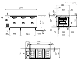
SUR-1871HP(AUH)-NNN [DRAWER TYPE]
