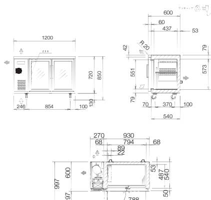
BR-1261HP(AUH [SLIMLINE TYPE]
