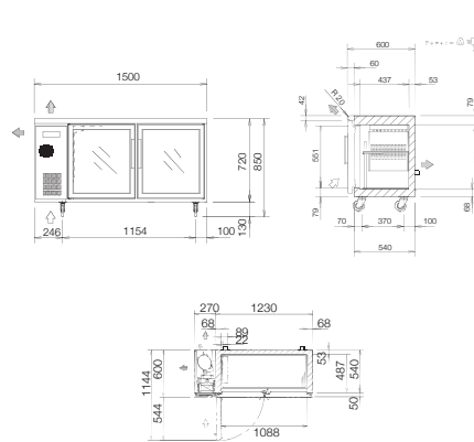
BR-1561HP(AUH [SLIMLINE TYPE])
