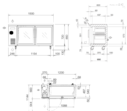
BR-1571HP(AUH) [LARGE CAPACITY TYPE]
