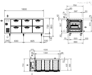
SUR-1871HP(AUH)-NNN [DRAWER TYPE]
