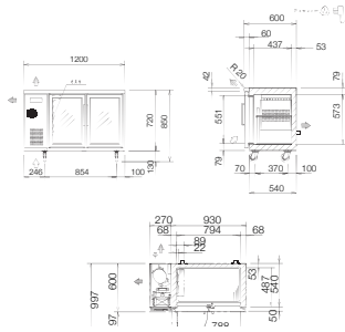
BR-1861HP(AUH) [SLIMLINE TYPE]
