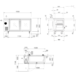
SUR-1871HP(AUH)-NNN [DRAWER TYPE]
