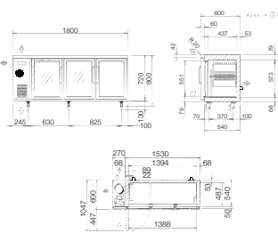
BR-1861HP(AUH) [SLIMLINE TYPE]
