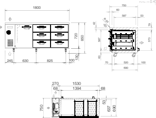
SUR-1871HP(AUH)-DWW [DRAWER TYPE]
