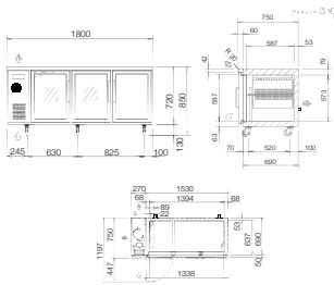
BR-1871HP(AUH) [LARGE CAPACITY TYPE]
