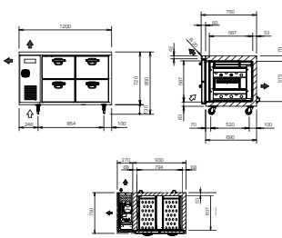
SUR-1271HP(AUH)-NN [DRAWER TYPE]
