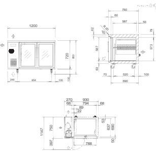
BR-1871HP(AUH) [LARGE CAPACITY TYPE]
