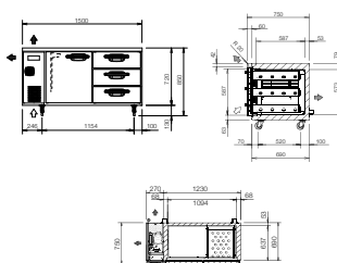
SUR-1571HP(AUH)-DW [DRAWER TYPE]
