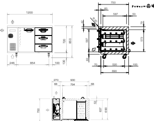
SUR-1271HP(AUH)-DW [DRAWER TYPE]
