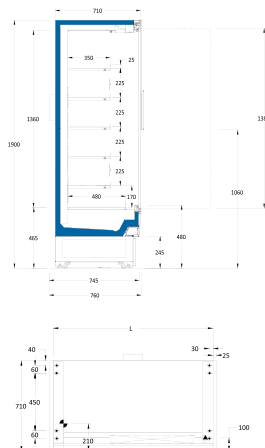
SGND193S HINGED
