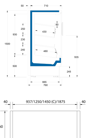
SGND153S SLIDING
