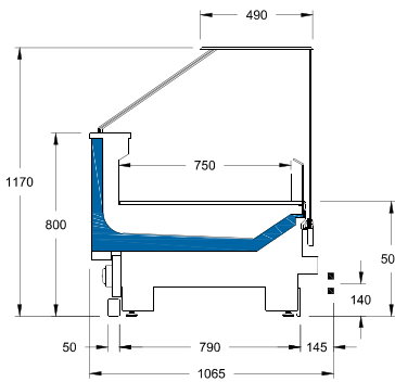
PDM11F5R-nX Serviced Deli Display Cabinet
