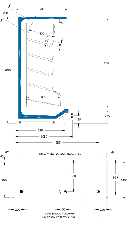
PMM20F3P-nP Multideck Door Produce
