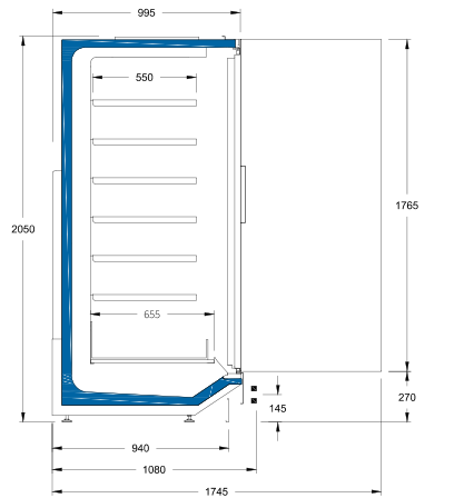
PGL20F3R-nZ Multideck Glass Door Freezer Frozen Food
