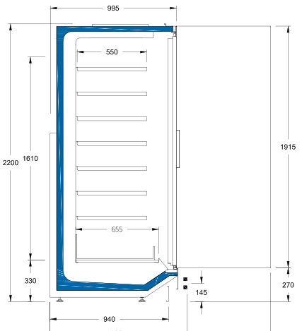
PGL22F3R-nZ Multideck Glass Door Freezer Frozen Food
