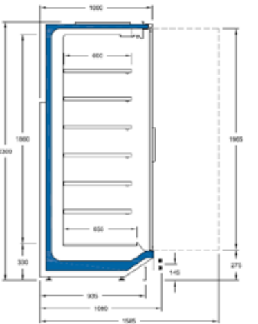
PMM23F3R4 Multideck Liquor
