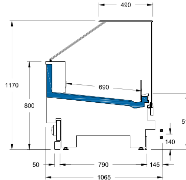
PCM11F5T-nF Serviced Cold Plate Cabinet Seafood
