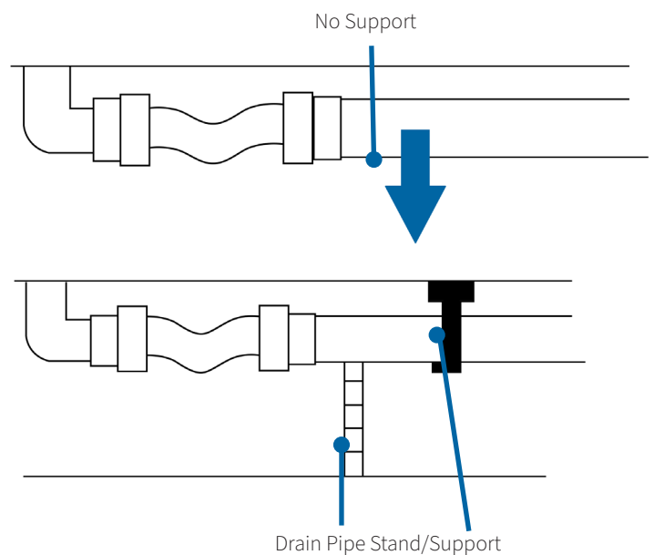
FIGURE 3AD- Drain Tap Orientation
