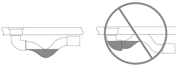
FIGURE 3AC- Drain Tap Orientation
