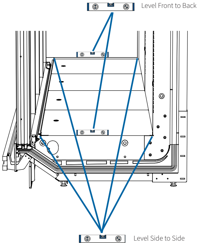
FIGURE 3C - Levelling Case
