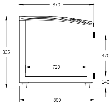
ARCH250-DTVS ARCH220-DTVS ARCH170-DTVS
