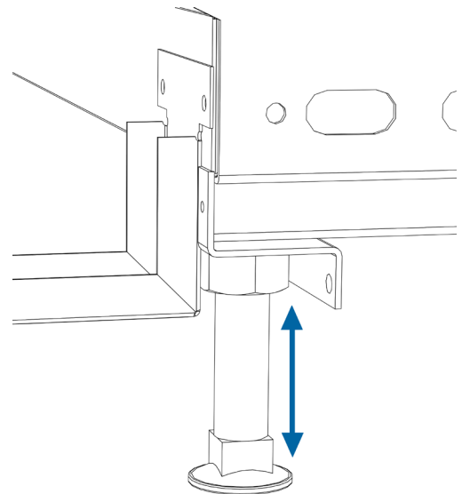
FIGURE 3B - Levelling Feet
