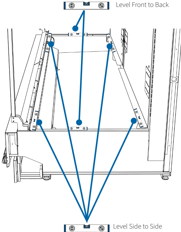
FIGURE 3C - Levelling Case
